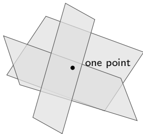
Three planes crossing at a single point: the one-solution case.
